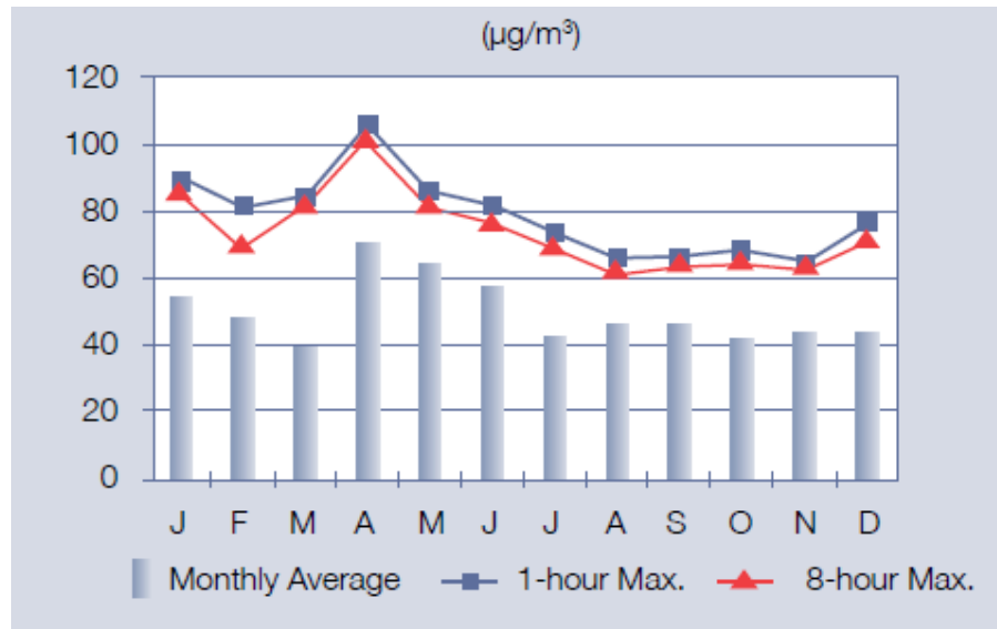
Figure 2.2-14 Summary of Inuvik 2008 O 3 Data
