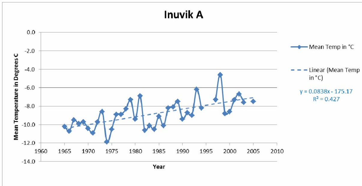
Figure 2.3-7 Inuvik A - Temperature in Degrees C Trend
