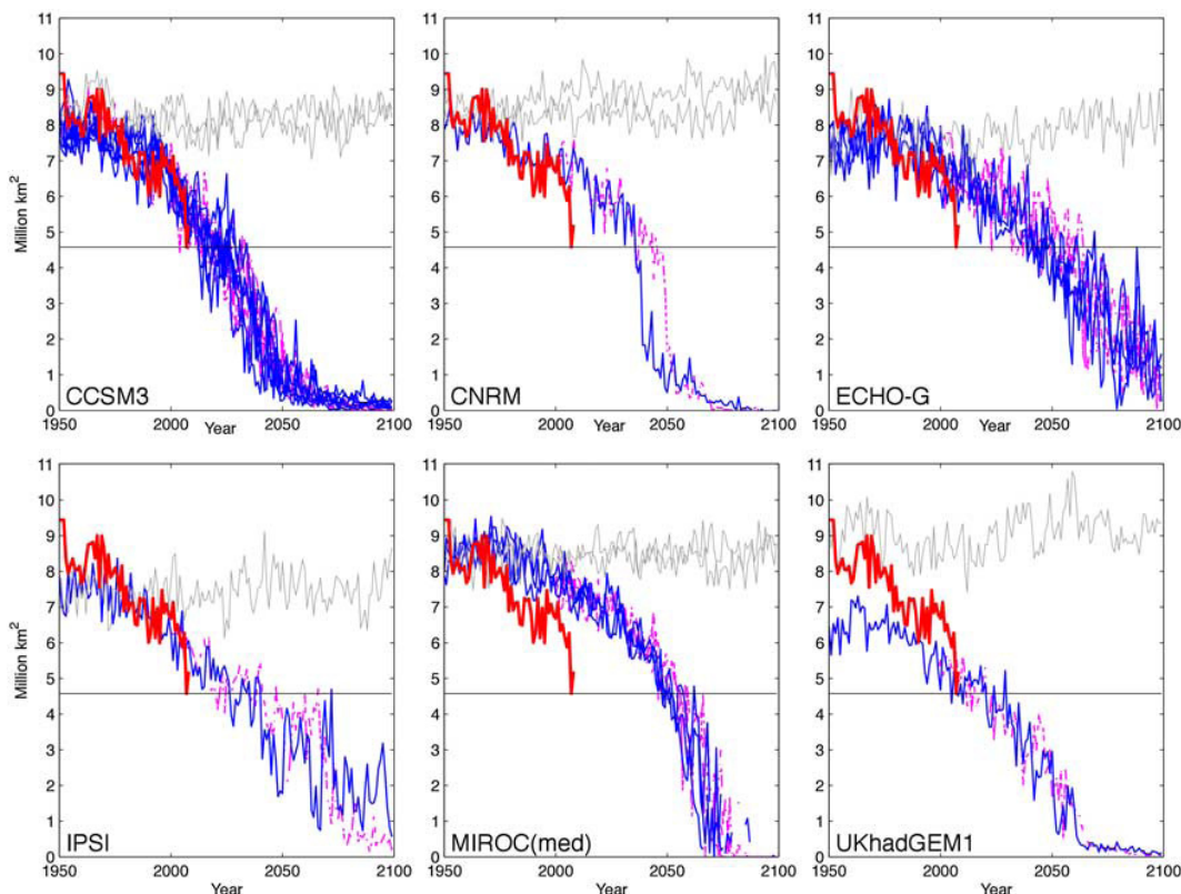
Figure 2.4-6 Modelled Future Sea-Ice Extent By Six Different Models
