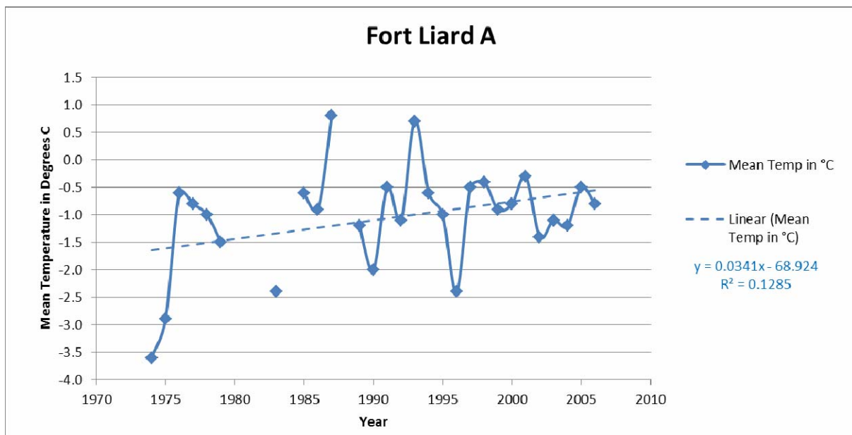
Figure 2.3-8 Fort Liard A - Temperature in Degrees C Trend
