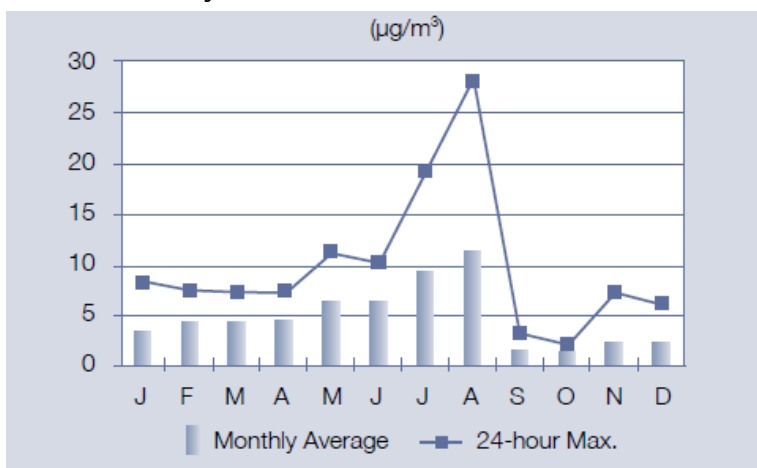
Figure 2.2-6 Summary of Fort Liard PM 2.5 Data for 2008
