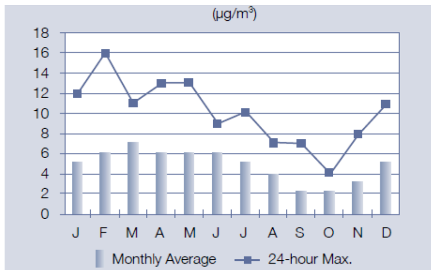
Figure 2.2-4 Summary of Inuvik PM 2.5 Data for 2008
