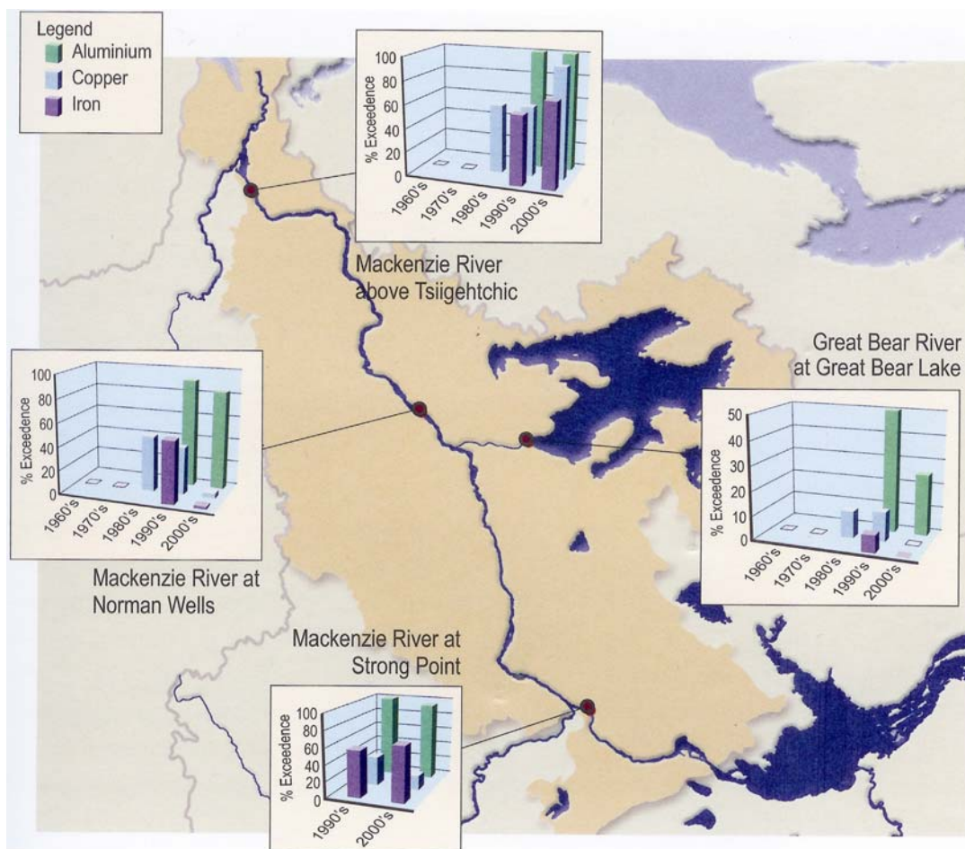
Figure 3.2-4 Temporal Metal (Aluminium, Iron, Copper) Monitoring and Exceedances from Various Locations Along the Mackenzie River and Great Bear River
