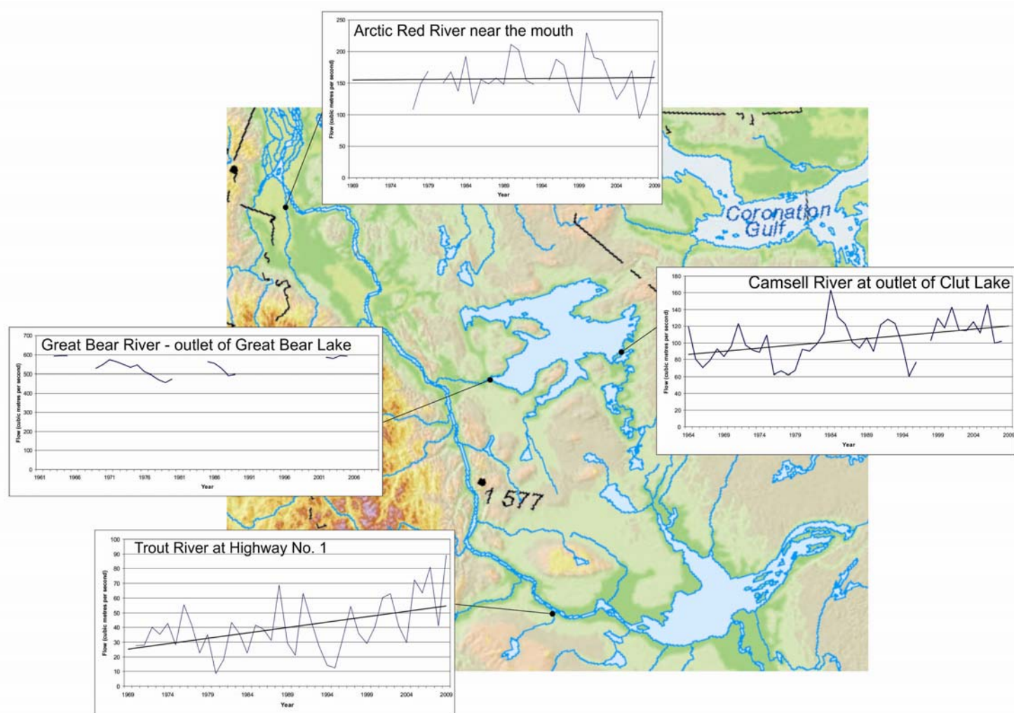
Figure 3.2-7 Average Annual Flow in the Mackenzie River Basin
