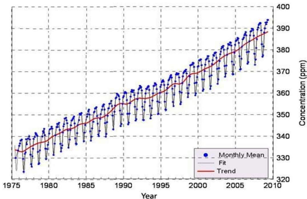
Figure 2.4-3 Trends in Atmospheric Carbon Dioxide Levels at Monitoring Stations in Nunavut
