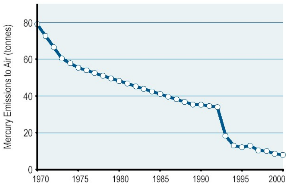
Figure 3.3-8 Decline in Canadian Anthropogenic Mercury Emissions Between 1970 And 2000
