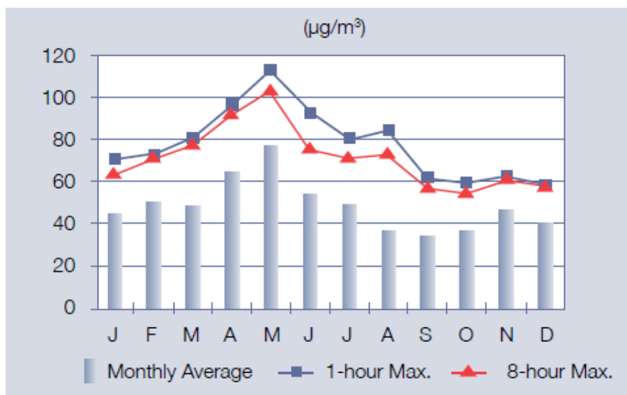
Figure 2.2-13 Summary of Yellowknife 2008 \text{O}_3 Data
