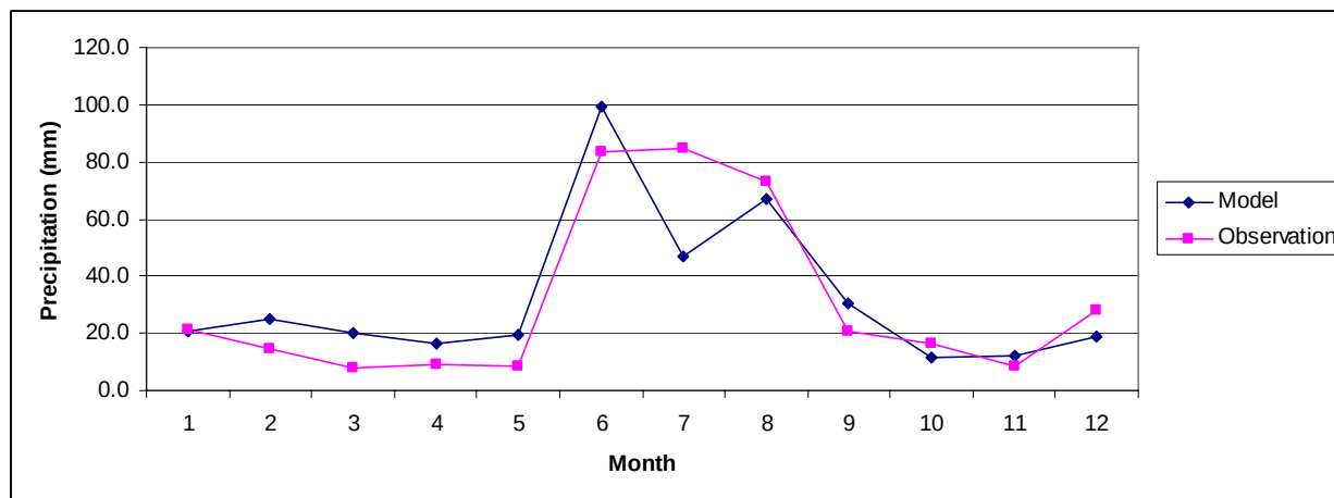
Figure 2.3-17 Monthly Total Precipitation - Norman Wells 2009
