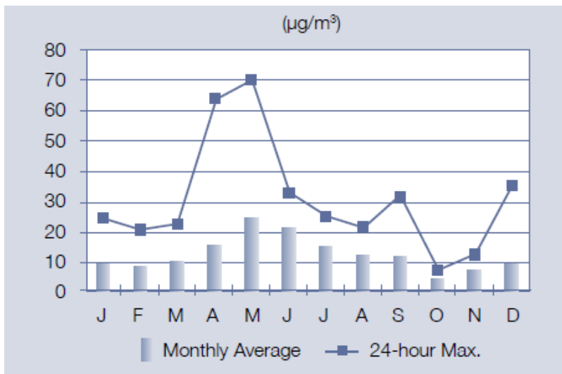
Figure 2.2-5 Summary of Inuvik PM 10 Data for 2008
