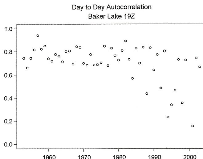
Figure 2.4-1 Daily Temperature Persistence at Baker Lake
