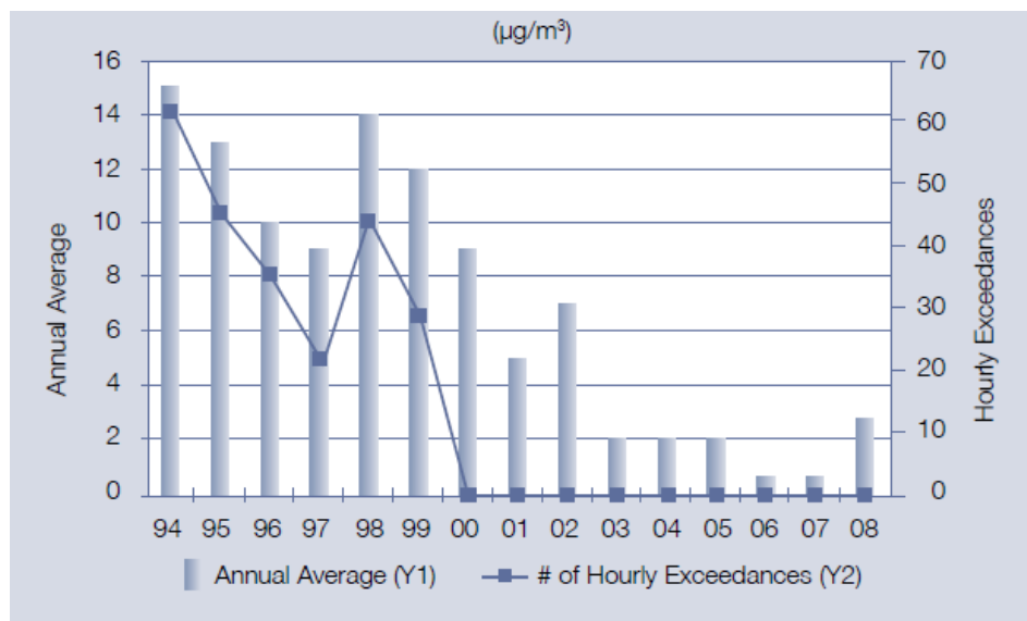
Figure 2.2-9 Summary of Yellowknife Annual Average SO 2 Data and Number of Exceedances of Hourly Standard
