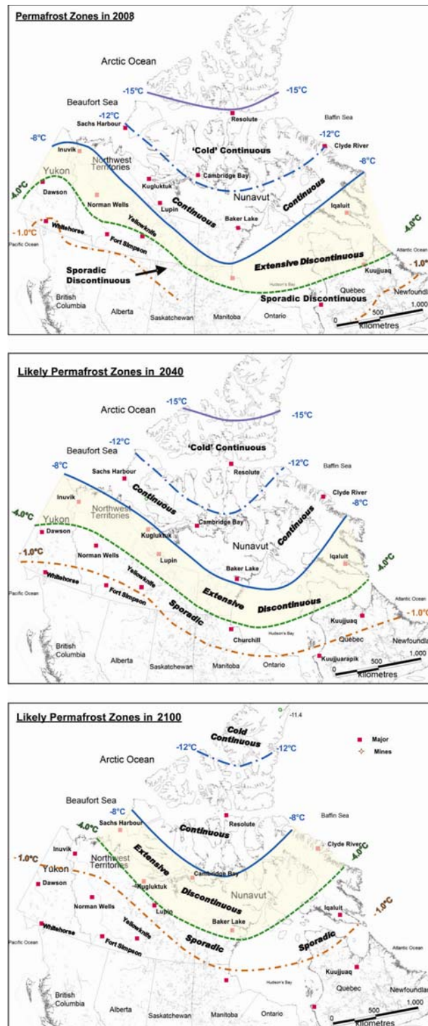
Figure 6.1-5 Predicted Changes of Permafrost Zones with Time Based on Mean Annual Air Temperature Increases and Constant Climate Warming Rate (Holubec & D' Uva 2011)
