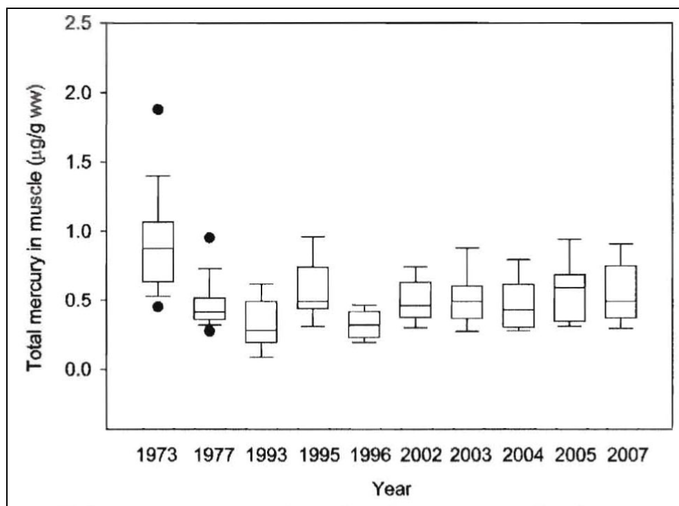
Figure 4.2-3 Total Mercury in the Muscle of Adult Ringed Seals Aged 7 – 36 Years from Ulukhaktok, NWT (1973-2007)
