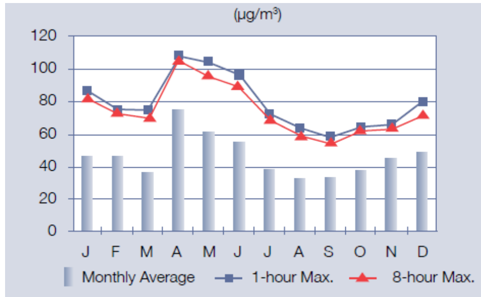
Figure 2.2-16 Summary of Norman Wells 2008 O 3 Data
