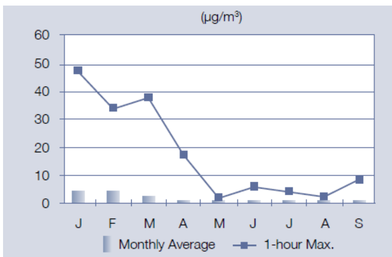
Figure 2.2-11 Summary of Inuvik 2008 NO 2 Data
