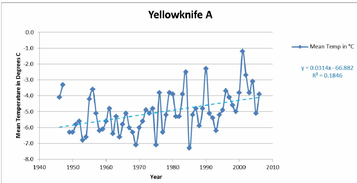
Figure 2.3-6 Yellowknife A - Temperature in Degrees C Trend
