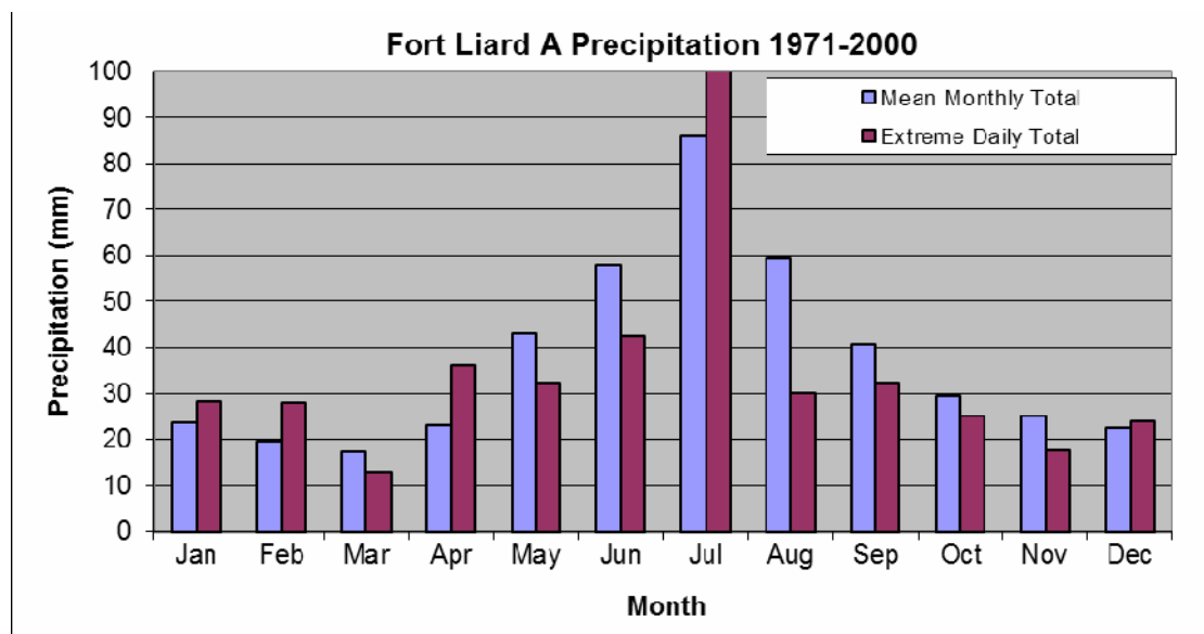
Figure 2.3-12 Climate Normal - Fort Liard A – Monthly Precipitation
