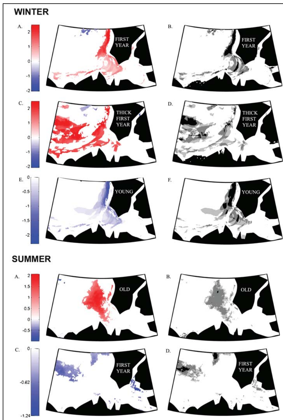
Figure 4.2-4 Winter and Summer Sea Ice (left) CONCENTRATION TREND (% per year) 1980-2004, (right) STATISTICAL SIGNIFICANCE (99% black, 95% dark grey, 90% light grey)
