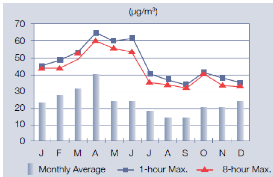
Figure 2.2-15 Summary of Fort Liard 2008 O 3 Data
