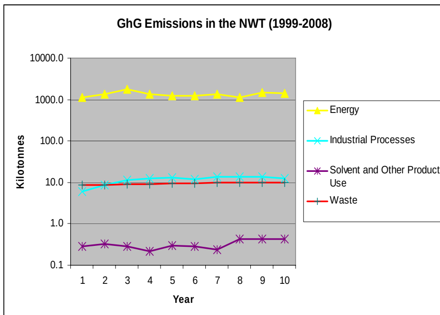
Figure 2.4-4 Northwest Territories GHG Emissions (1999-2008)
