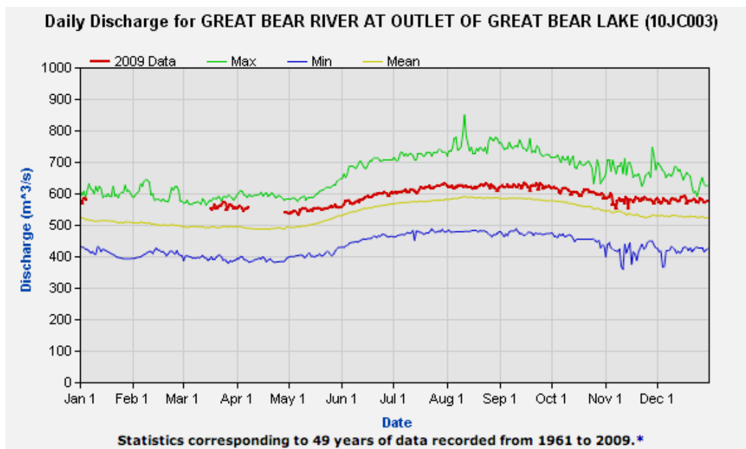
Figure 3.2-8 Annual Hydrograph of the Great Bear River, 1961-2009
