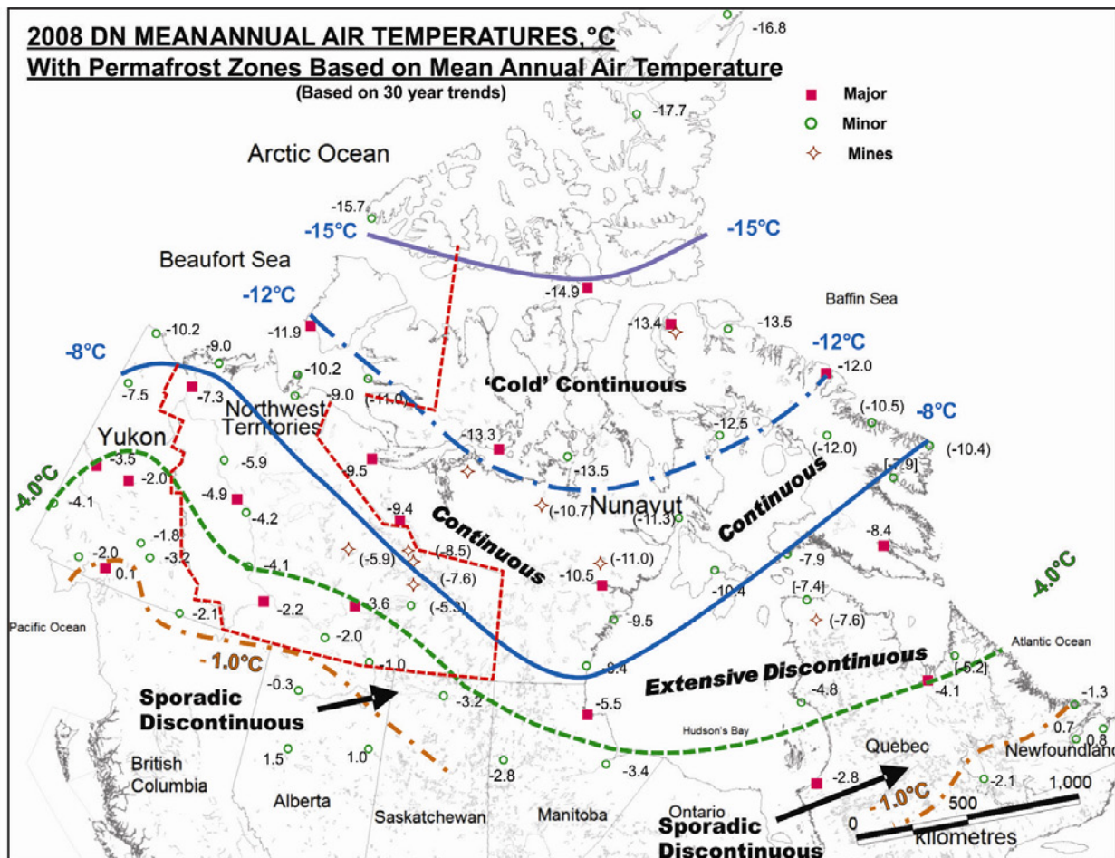
Figure 6.1-1 Permafrost Conditions Based on 2008 Mean Annual Air Temperatures (Holubec & D’Uva 2011)
