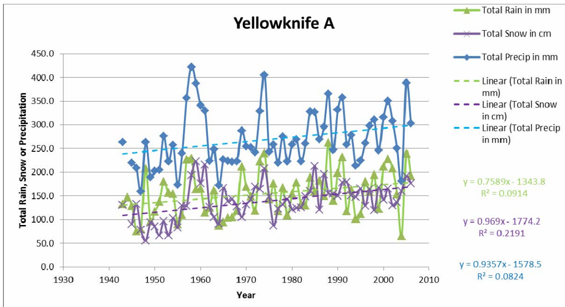
Figure 2.3-14 Yellowknife A - Precipitation Trend
