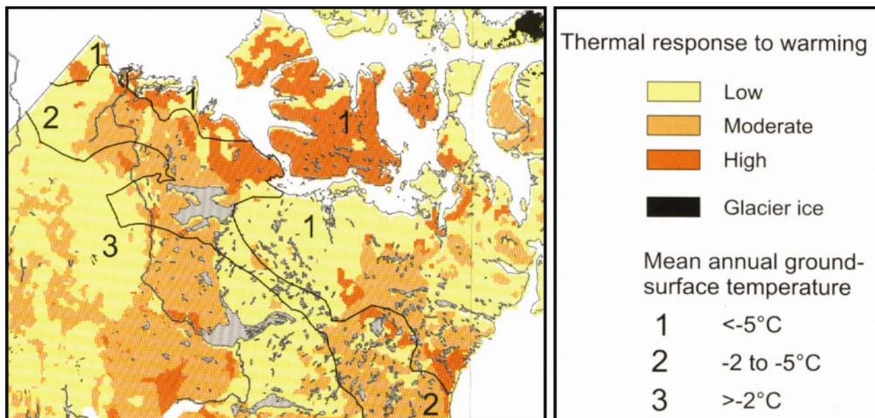
Figure 6.4-2 Relative Thermal Response of Permafrost to Climate Warming from GSC Bulletin 579 (Smith & Burgess 2004)
