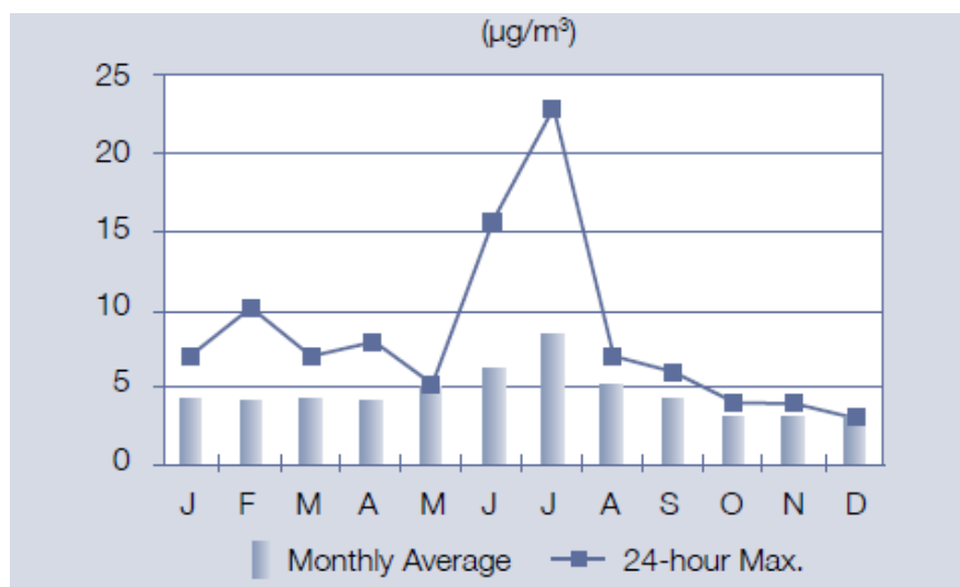
Figure 2.2-8 Summary of Norman Wells PM 2.5 Data for 2008
