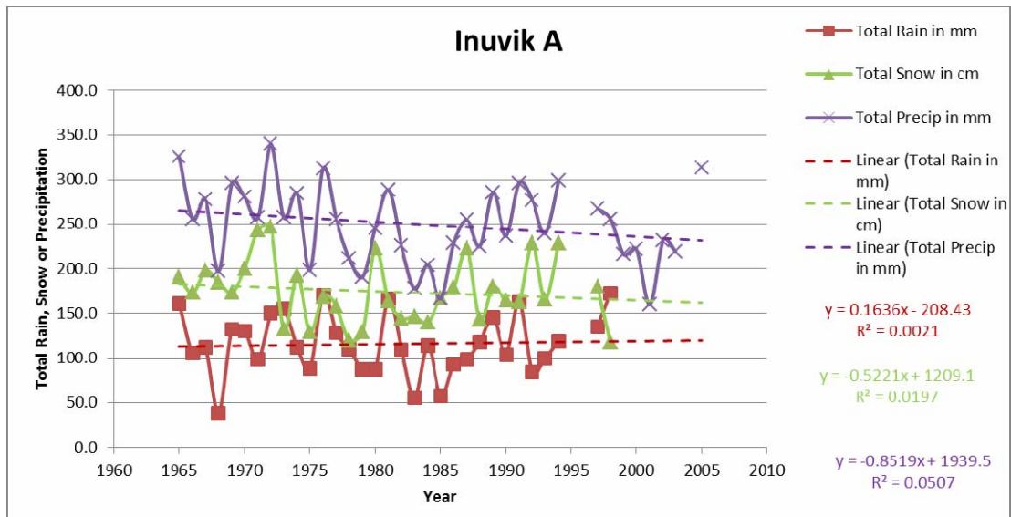
Figure 2.3-15 Inuvik A - Precipitation Trend
