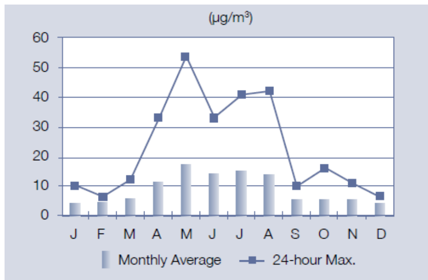
Figure 2.2-7 Summary of Fort Liard PM 10 Data for 2008
