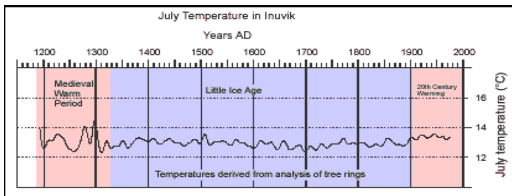
Figure 2.4-2 Historic Record of July Temperatures In Inuvik
