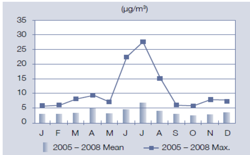
Figure 2.2-3 Summary of Yellowknife PM 2.5 Data for the 2005-2008 Period
