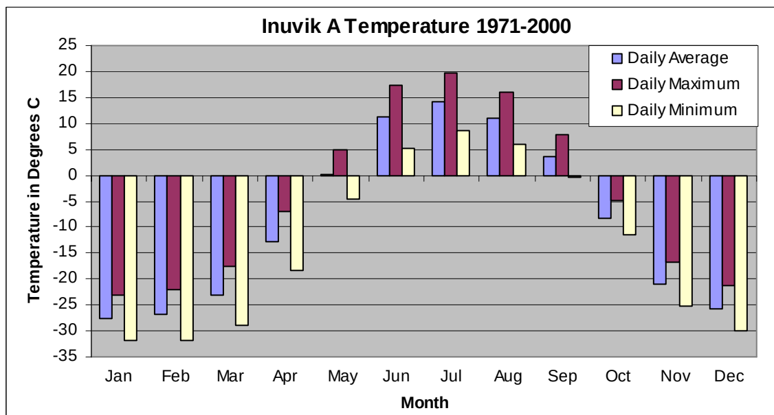
Figure 2.3-3 Climate Normal - Inuvik A - Monthly Mean Temperatures
