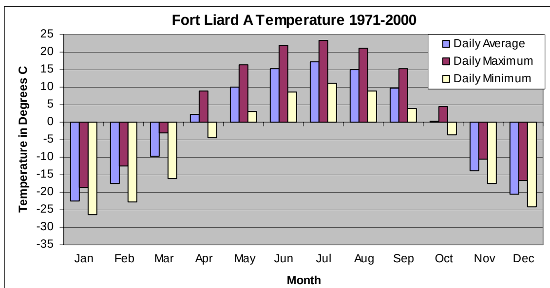
Figure 2.3-4 Climate Normal - Fort Liard A – Monthly Mean Temperatures
