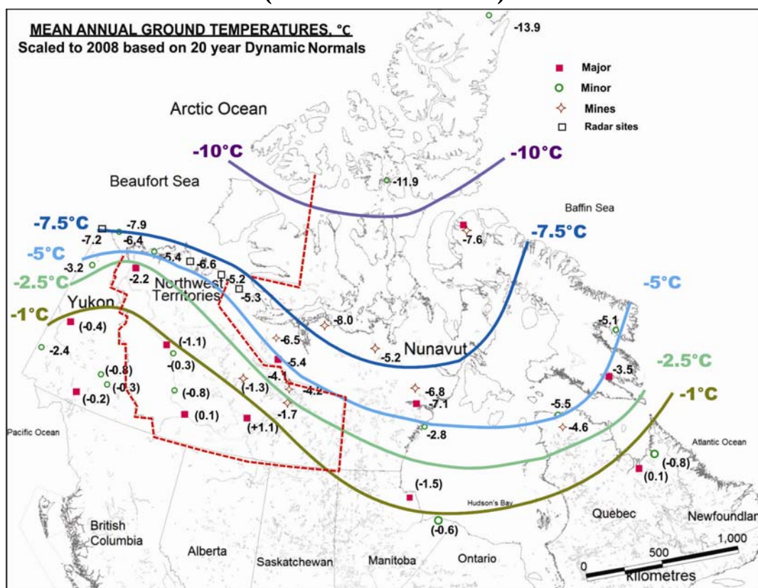
Figure 6.1-6 Ground Temperatures in NWT as Measured or Scaled to 2008 (Holubec & D’Uva 2011)
