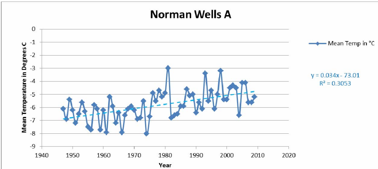
Figure 2.3-5 Norman Wells A - Temperature in Degrees C Trend
