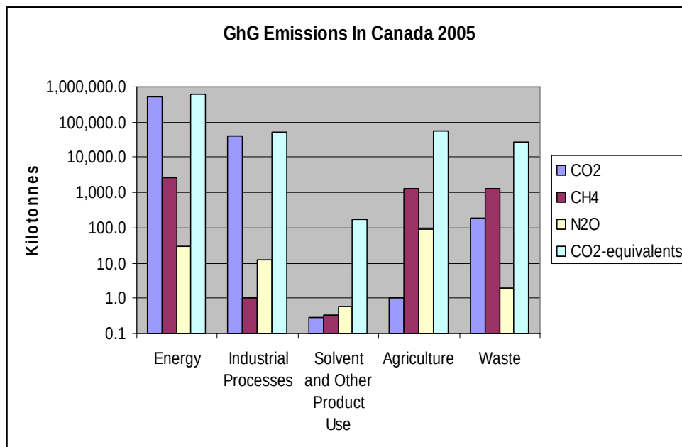
Figure 2.4-5 GHG Emissions (in Kilotonnes) for Canada in 2005
