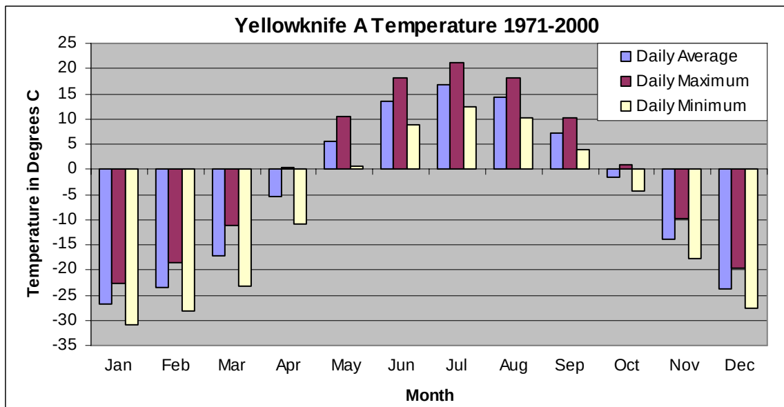
Figure 2.3-2 Climate Normal - Yellowknife A – Monthly Mean Temperatures
