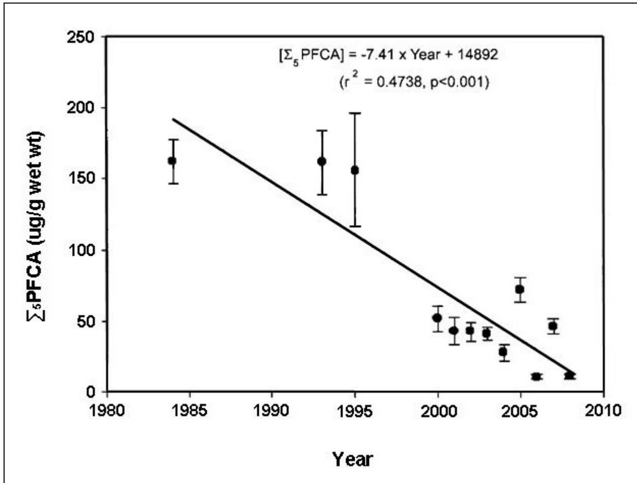
Figure 4.2-2 Temporal Trend of \Sigma 5 PFCA Concentrations in the Liver of Belugas from Hendrickson Island
