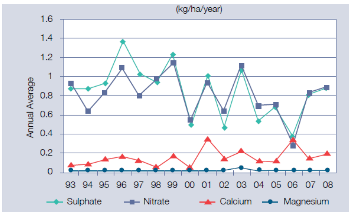
Figure 2.2-19 Acid Deposition at Snare Rapids
