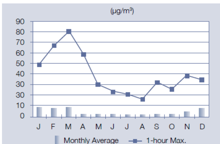
Figure 2.2-10 Summary of Yellowknife 2008 NO 2 Data
