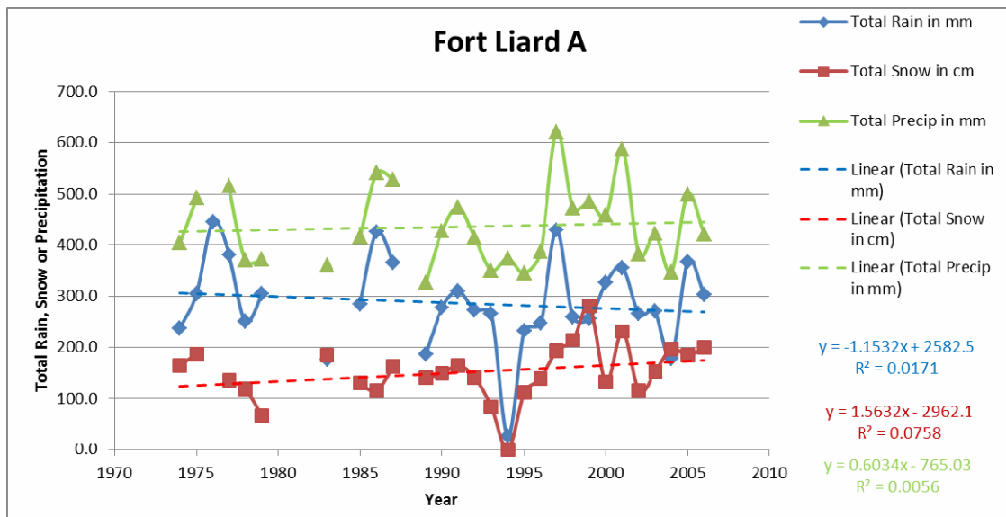
Figure 2.3-16 Fort Liard A - Precipitation Trend
