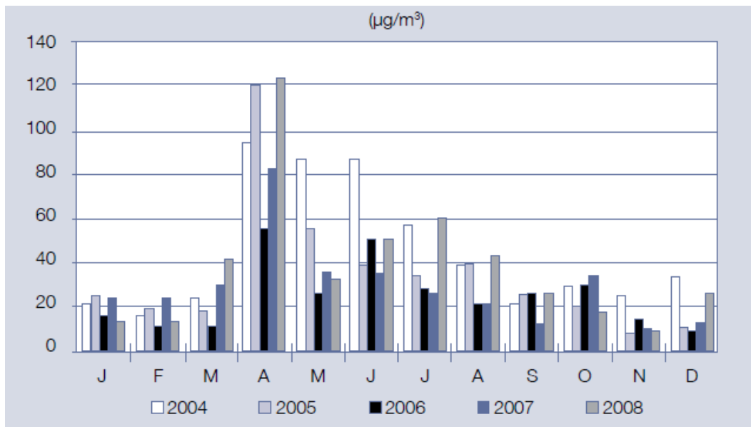
Figure 2.2-2 Monthly TSP in Yellowknife for the 2004-2008 Period
