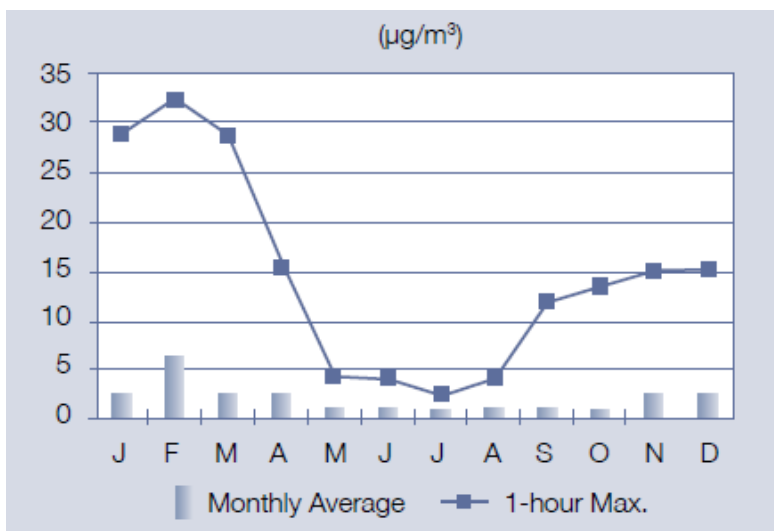
Figure 2.2-12 Summary of Norman Wells 2008 NO 2 Data
