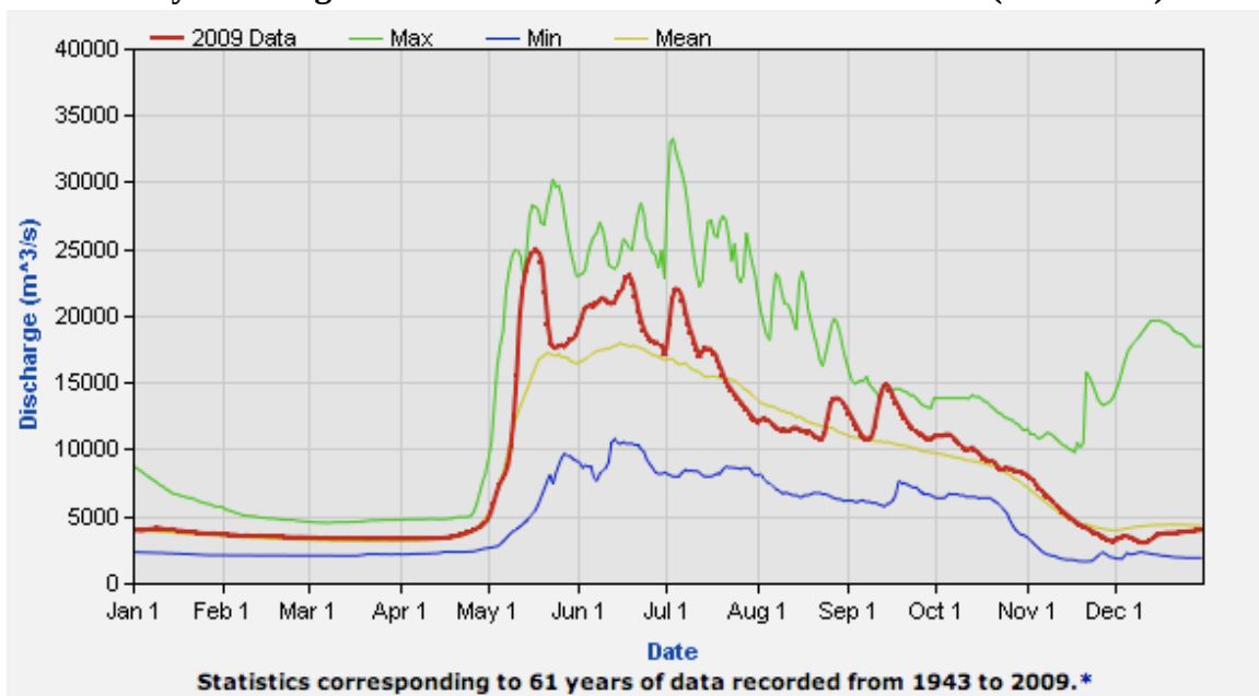
Figure 3.2-6 Daily Discharge for the Mackenzie River at Norman Wells (1943-2009)
