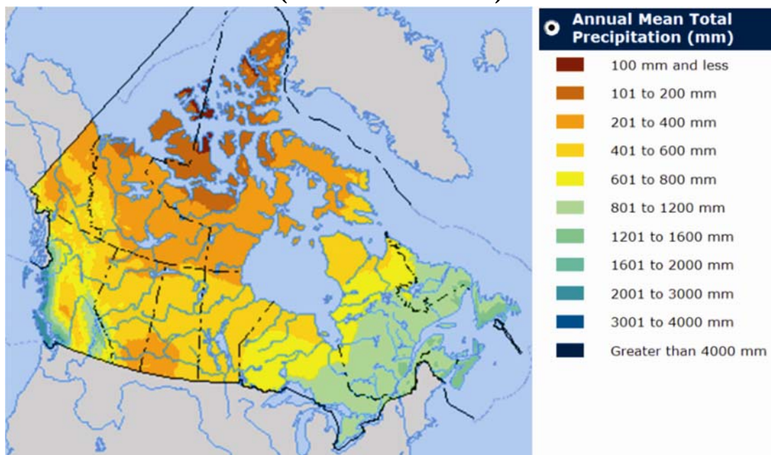
Figure 6.3-1 Annual Mean Total Precipitation (Mm) For 1971-2008 Period (Atlas of Canada 2009)
